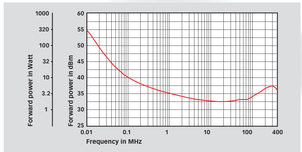
BCI application: Typical required forward power to inject 100 mA (100 dB \mu A)
